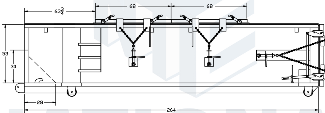
DRIVER'S SIDE ELEVATION VIEW.
