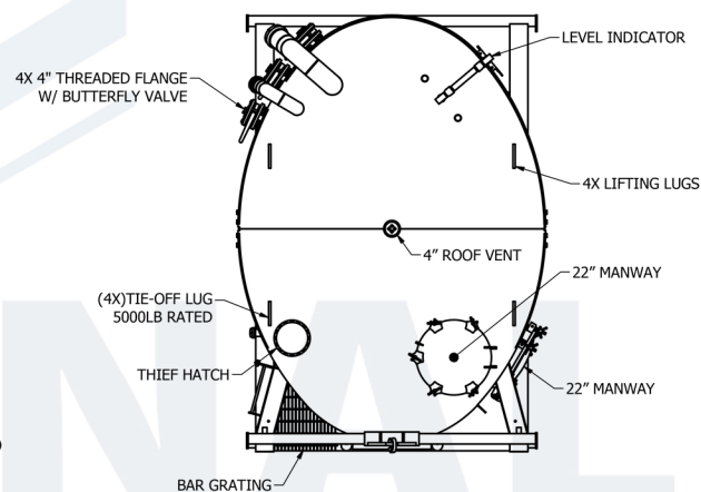
SECTION B-B SCALE 1 / 30
